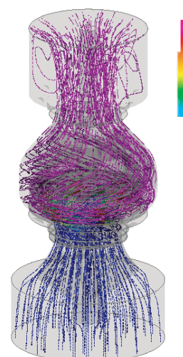
360° Hydraulic Balance
